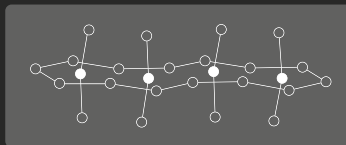
Coordination of protactinium (solid circles) and halogen atoms (open circles) in protactinium(V) fluoride or chloride.
